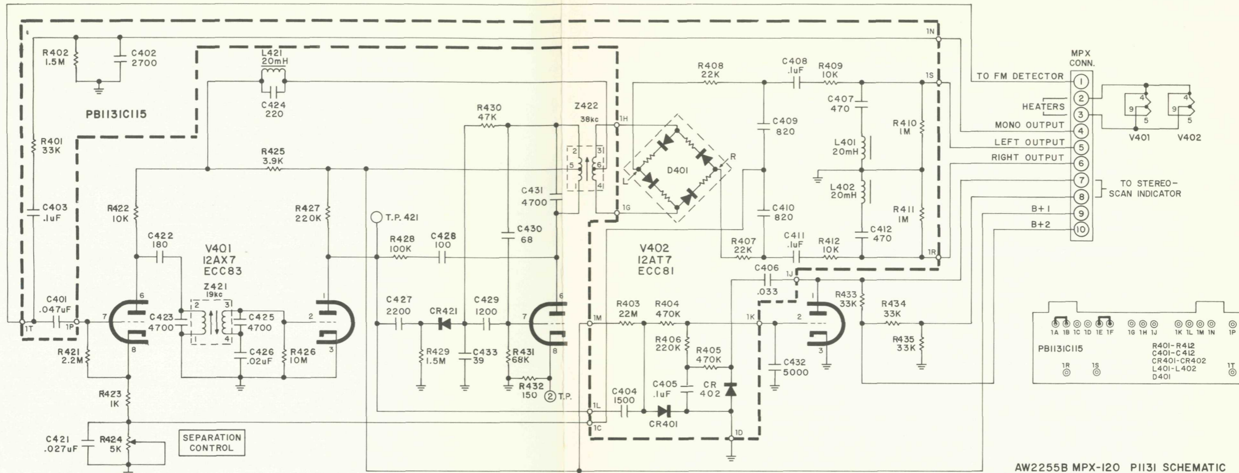
AW2255B MPX-I20 P1131 SCHEMATIC
